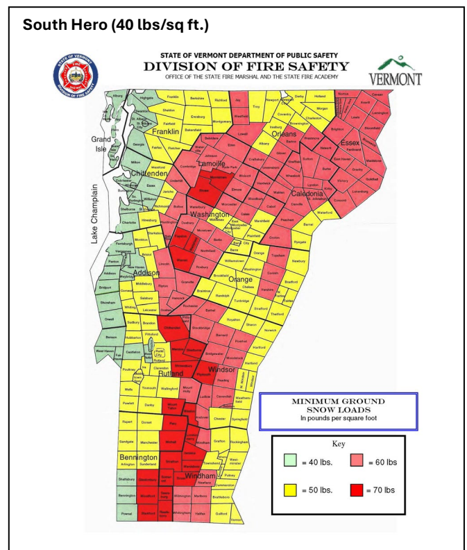
Figure 6: Minimum Snow Loads for Construction
