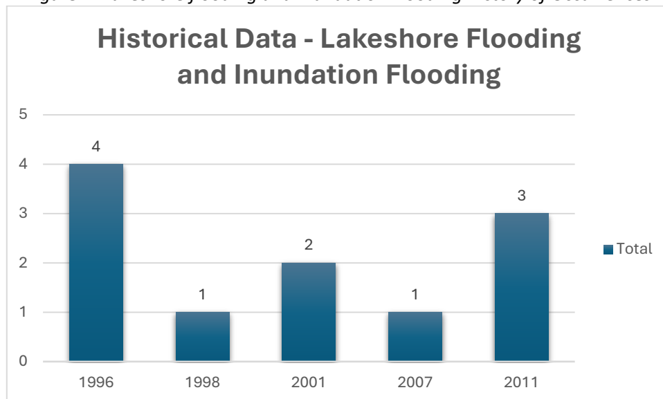
Figure 4: Lakeshore flooding and Inundation Flooding History of Occurrences
