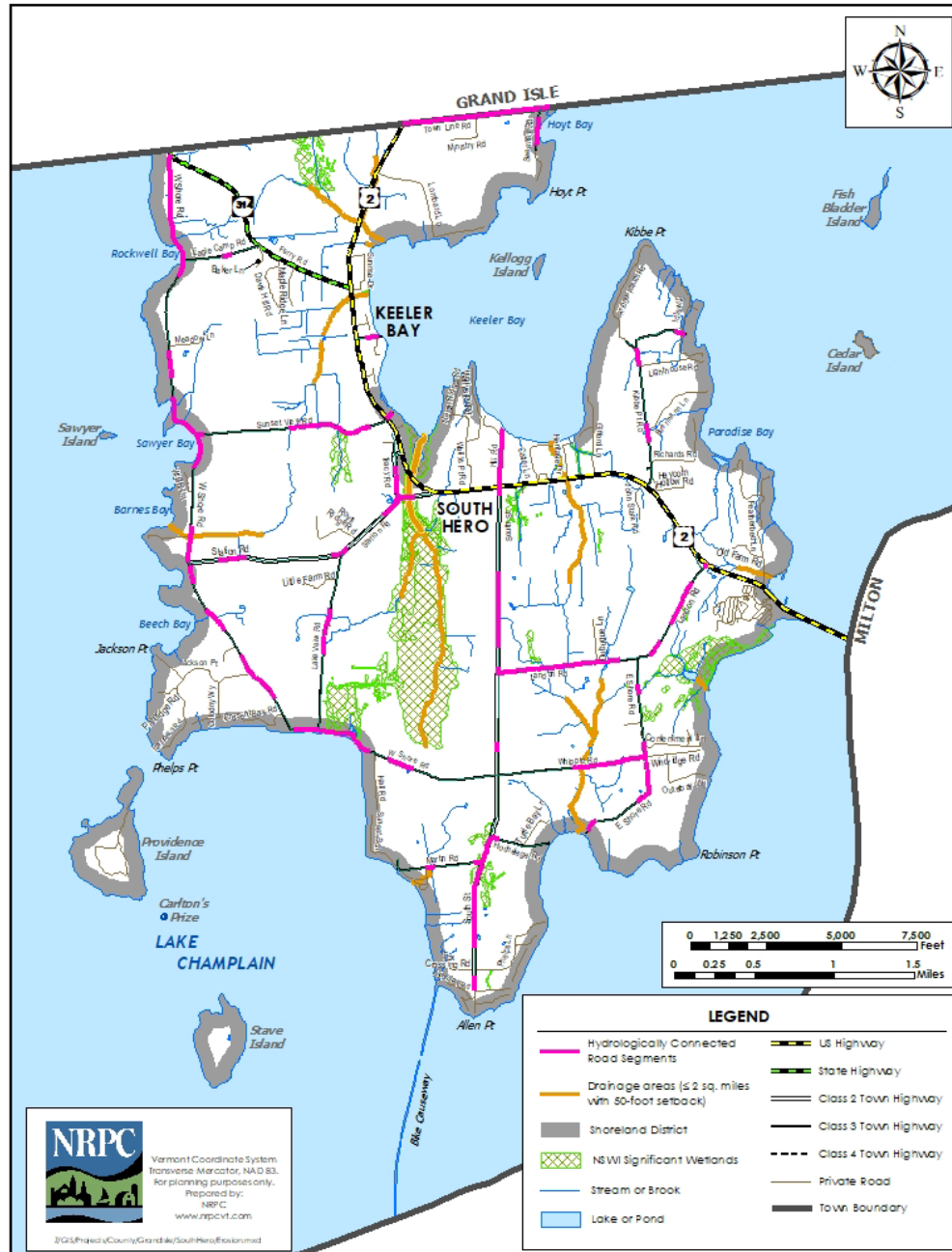
Figure 10: Grand Isle Erosion Risk Map
